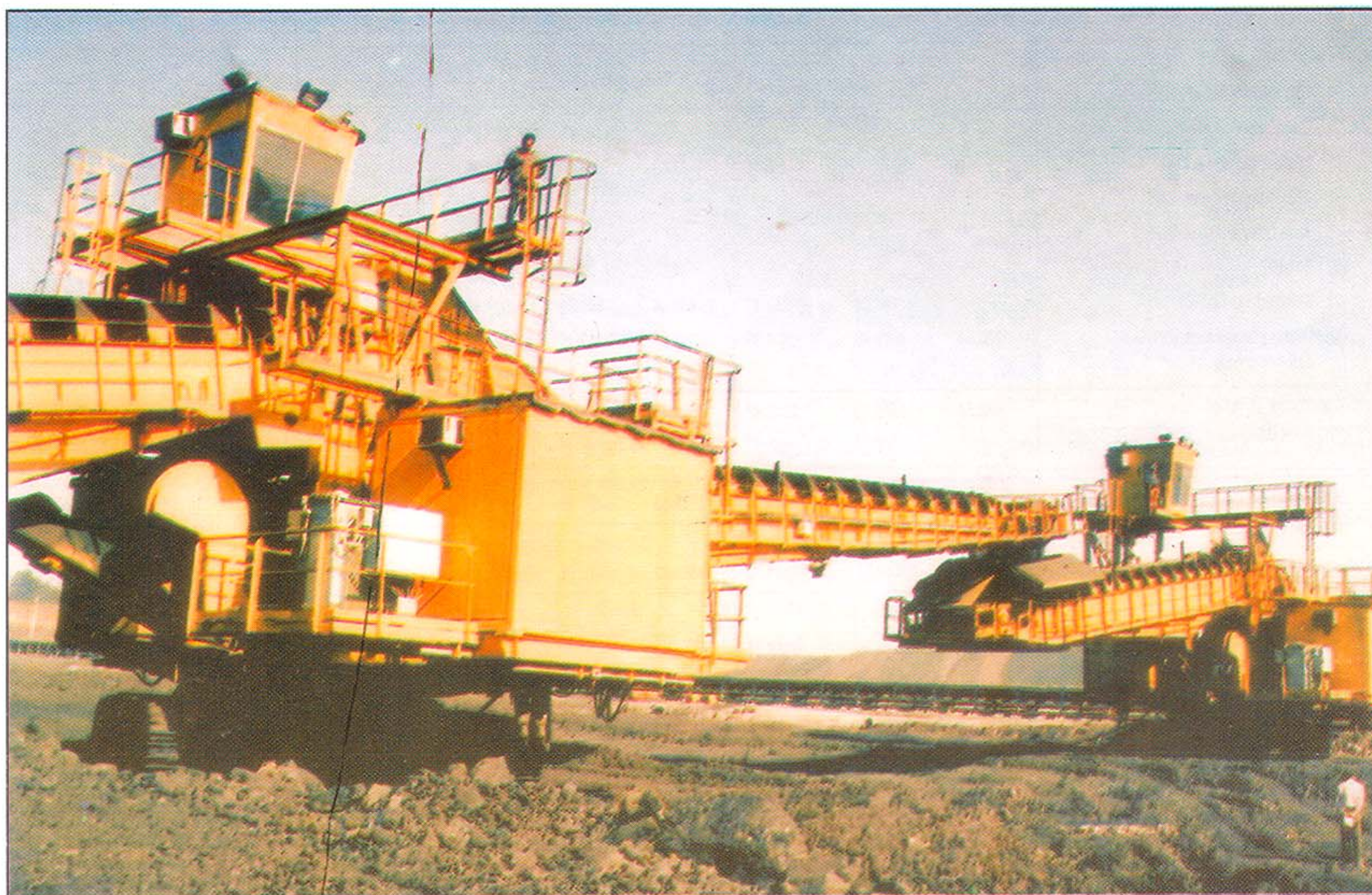
Modern opencast mining machine, In-Pit Coal Crusher in operation at Piparwar OCP
